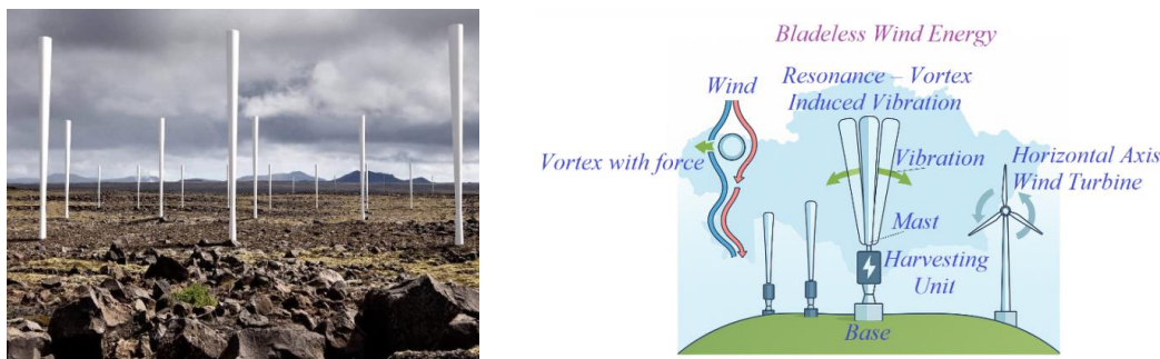
FIGURE 1. Schematic Representation of Vortex-Resonance-Based Bladeless Wind Energy Conversion
