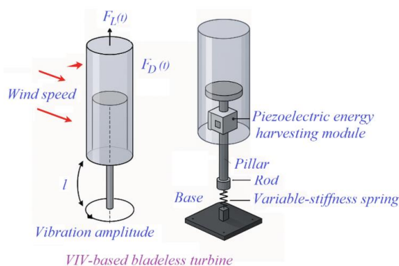
FIGURE 2. Structural and dynamic model of a VIV-based bladeless wind turbine
