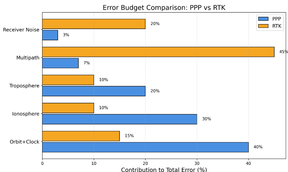
FIGURE 4. Error Structure in PPP and RTK Methods
