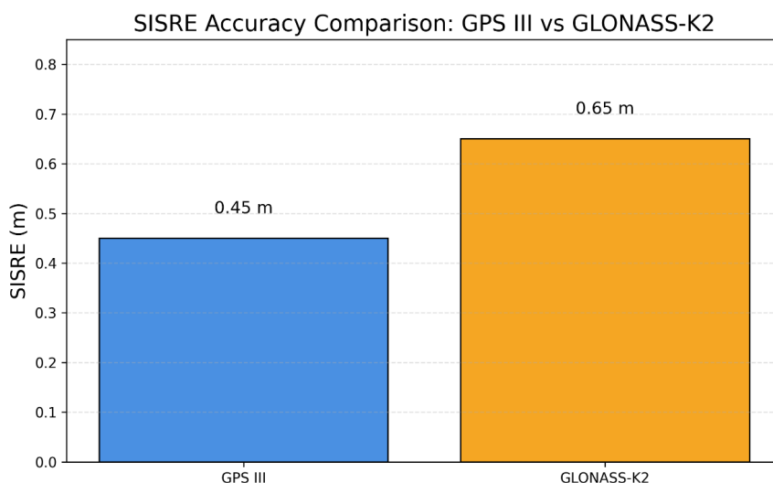
FIGURE 3. Signal-in-Space Range Error (SISRE): GPS III vs. GLONASS-K2
