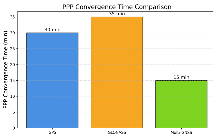
FIGURE 2. PPP Convergence Time for GPS, GLONASS, and Multi-GNSS
