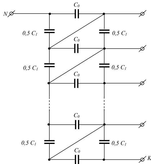
FIGURE 2. Equivalent capacitance scheme of a multilayer winding
