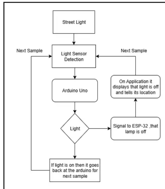
Figure 2: LIGHT SENSING MECHANISM
