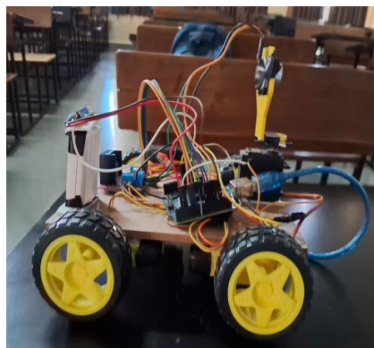
Figure 3- LIGHT INSPECTION VEHICLE (HARDWARE)
