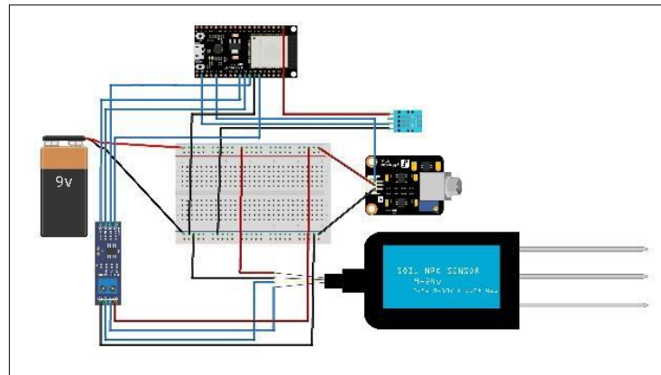
FIGURE. 3 HARDWARE SETUP
