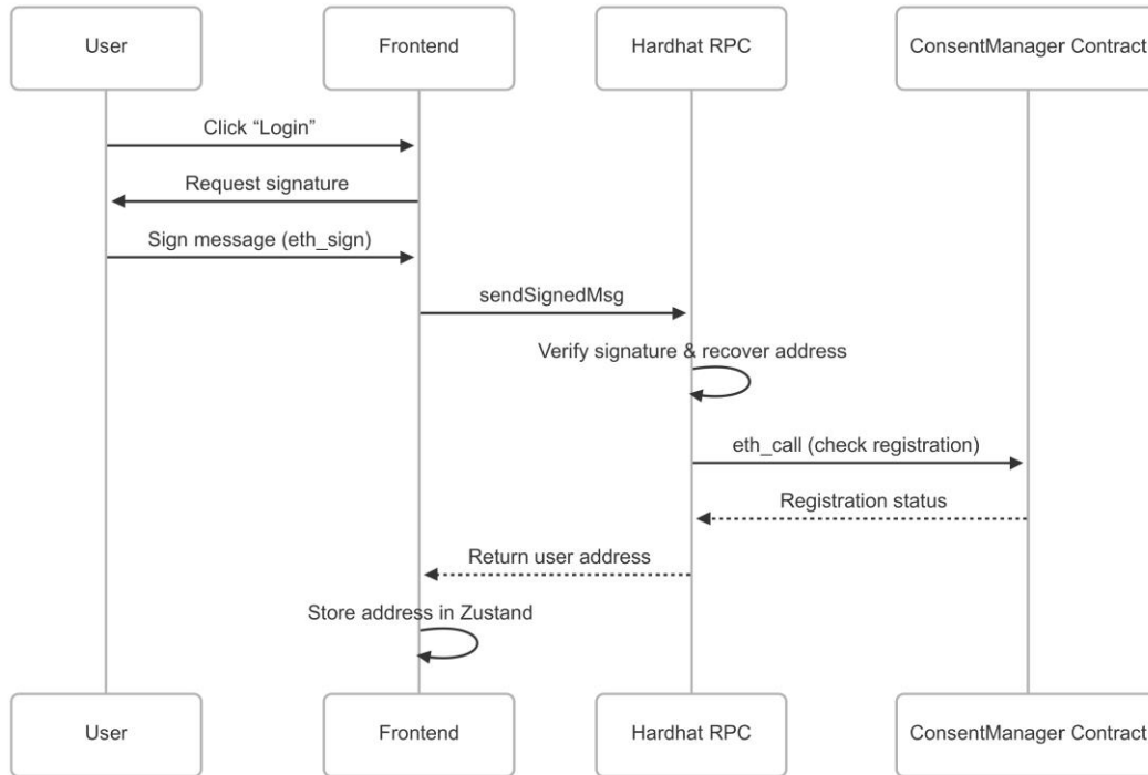
Fig. 3. authentication
