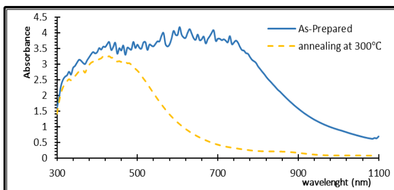
FIGURE 3. Absorption Spectrum versus wavelength Before and After Annealing
