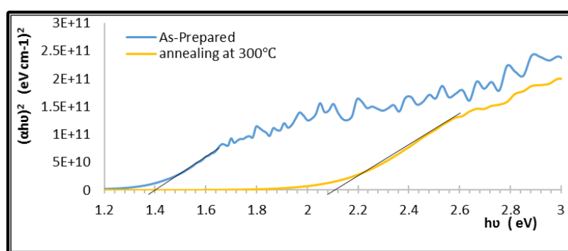
FIGURE 4. Variation (\alpha h\nu)^2 versus (h\nu) of SnSe thin film Before and After Annealing.
