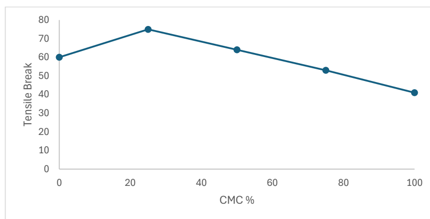
FIGURE 3. The relationship between adhesion strength and weight fraction increase of CMC.
