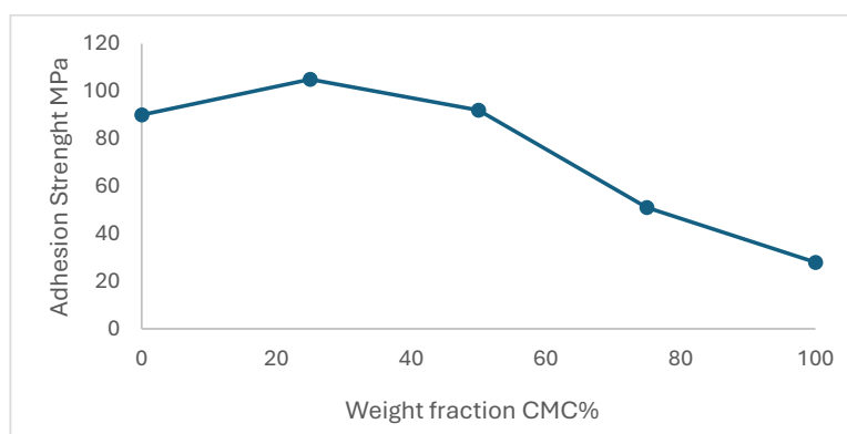
FIGURE 2. The relationship between adhesion strength and weight fraction increase of CMC%.
