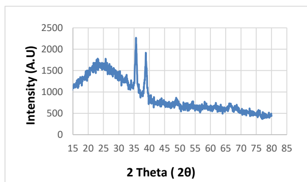
Fig. 2: XRD pattern for CuO NP synthesis by plasma jet
