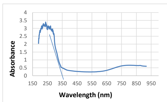
Fig. 5: CuO nanoparticles optical absorption spectra
