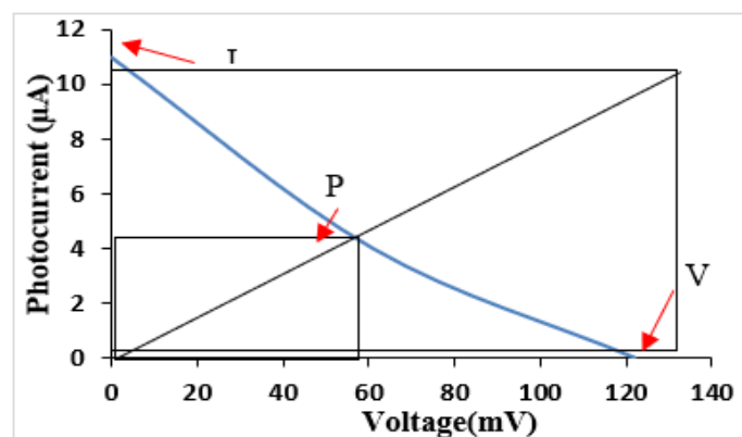
Fig. 9. Open-circuit voltage of the (Al/p-Si/p-CuO) heterojunction.
