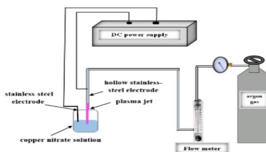
Fig.1: Plasma jet system
