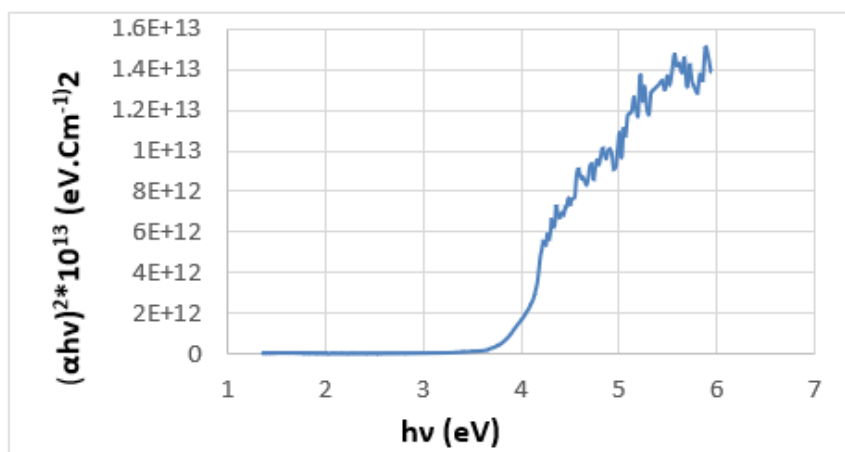
Fig. 6: Optical bandgap energy for CuO NPs.
