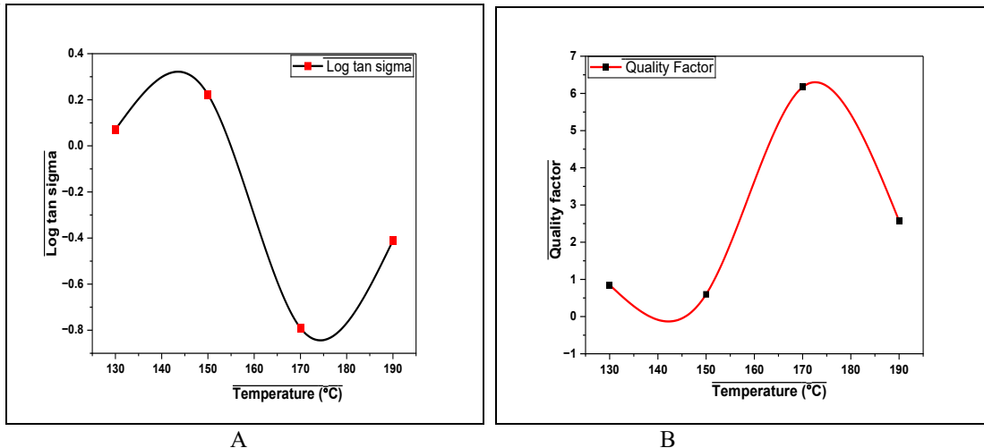
FIGURE 5. (A) Relationship between tan insulation Dissipation factor with changing temperature. (B) Relationship between the Quality factor with changing temperature.
