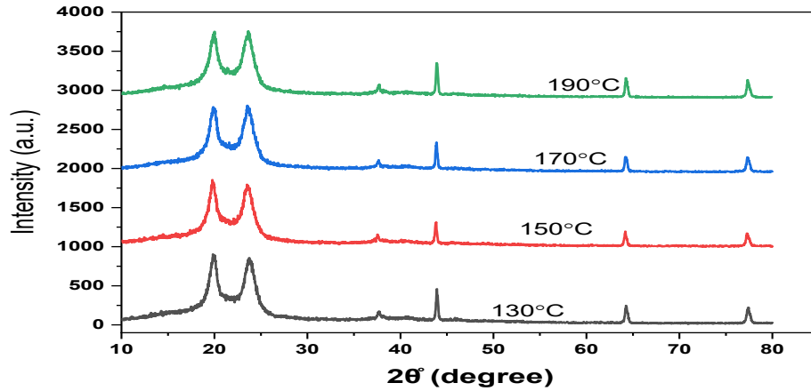
FIGURE 1. The XRD of Nylon.
