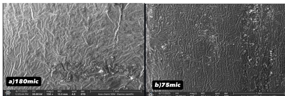
Figure 6 SEM micrographs of a -(UPE/ 180 MLP), b-(UPE/ 75 MLP)
