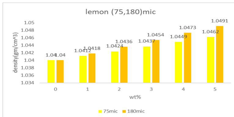
Figure2: densities values of UPE composites
