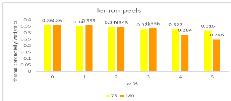
Figure 3 thermal conductivity values of UPE composites
