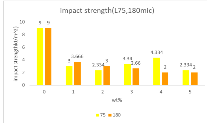
Figure 5: Impact strength values of UPE composites
