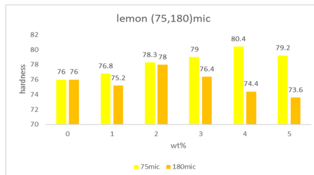
Figure 4 Hardness values of UPE composites
