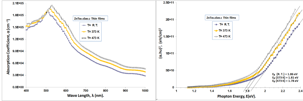
FIGURE 2. Variation in the absorption coefficient with \lambda for ZnTe 0.8 Se 0.2 at temperature (R.T, 373 and 473)
