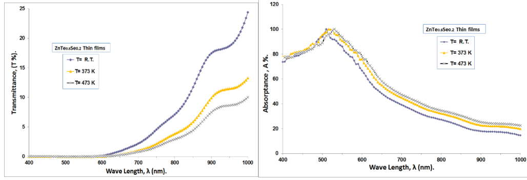
FIGURE 1. Transmittance and absorption spectrum of ZnTe 0.8 Se 0.2 at (R.T, 373 and 473) K
