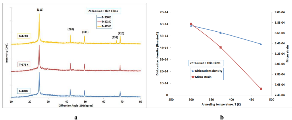
FIGURE 4a,b. X-ray diffraction for the \text{ZnTe} thin films at (R.T, 373 K and 473 K)
