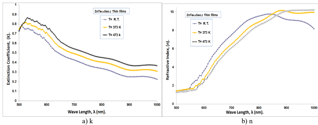
FIGURE 3a,b. Variation of the optical parameters k , n versus wavelength for \text{ZnTe}_{0.8}\text{Se}_{0.2} at temperature R.T, 373 and 473 K
