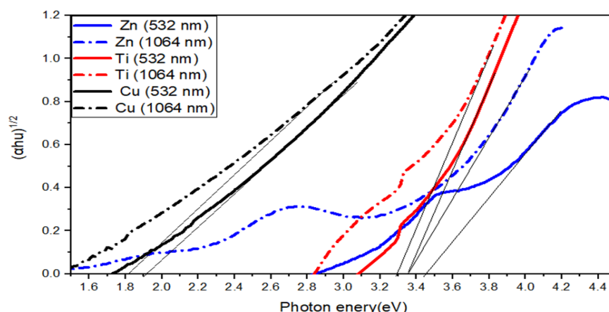
FIGURE 3. Energy gap of pulsed laser ablated samples in liquid medium: pure oxides (ZnO, \text{TiO}_2 , CuO) prepared at 532 nm, 1064 nm laser wavelengths.
