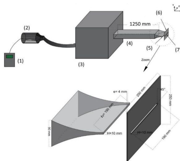
FIGURE 1. Schematic configuration (1) frequency chopper (2) compressor (3) damping volume (4) duct (5) rectangular nozzle (6) plate (7) slot.
