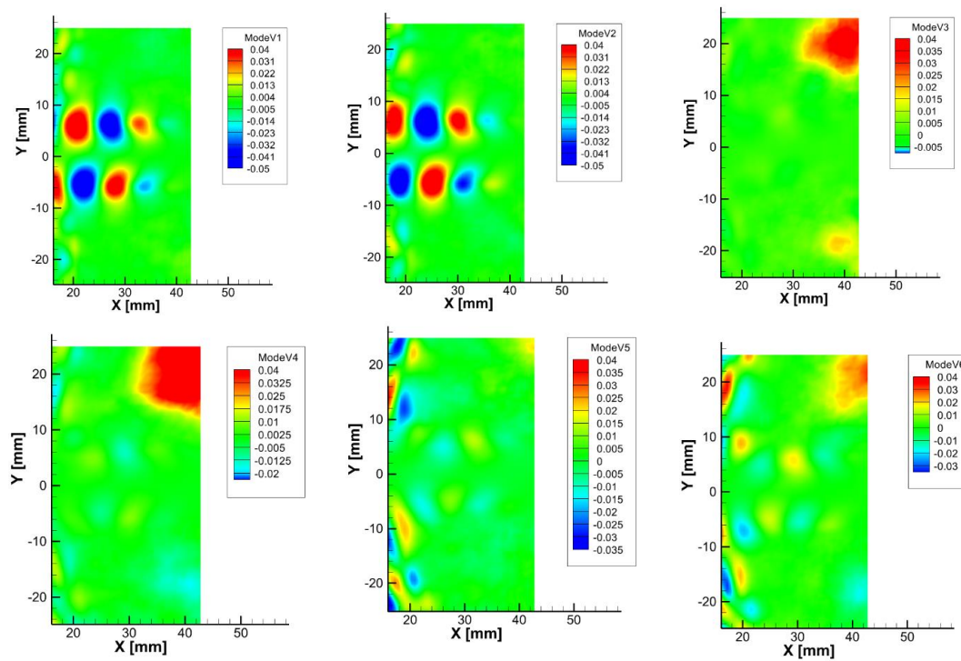
FIGURE 3. The first six POD mode.
