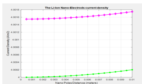
FIGURE 10. The achieved Li-Ion nano-electrodes current density ( i ) using Butler-Volmer and Fick equations model in time domain, for n/\eta=200/50=4 poles/volts
