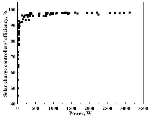
FIGURE 5. Efficiency curve of MPPT.
