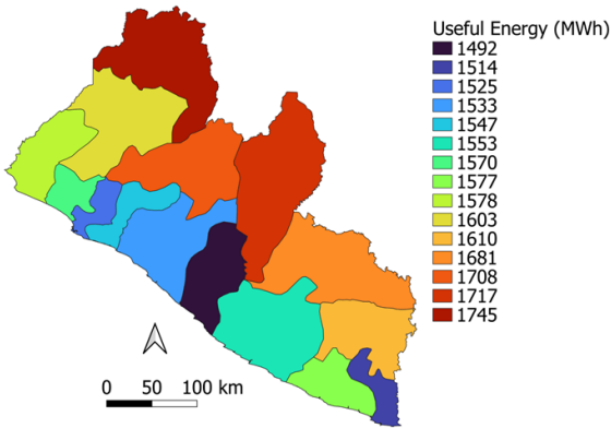
FIGURE 5. First year useful energy generation
