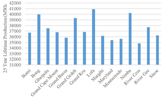
FIGURE 8. Useful energy over 25 years graph
