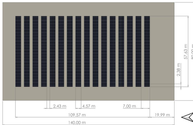
FIGURE 3. Solar Panel layout
