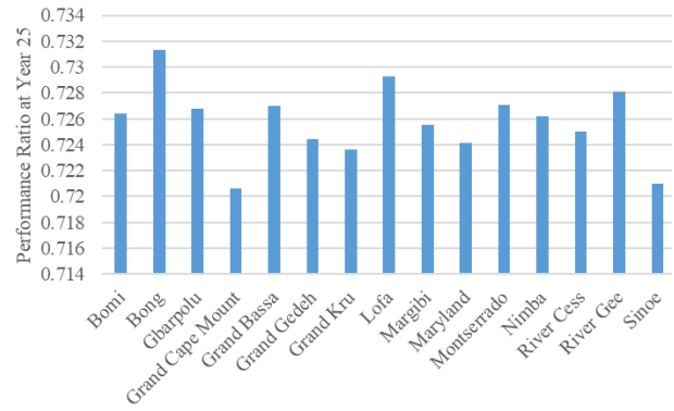
FIGURE 10. Performance Ratio at end of Project Life
